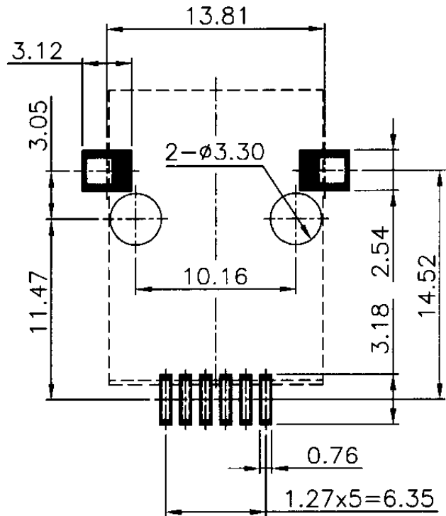
PCB LAYOUT/TOP VIEW
