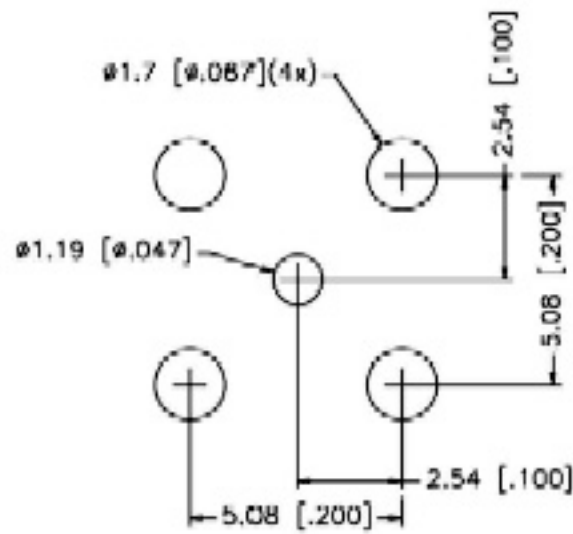
PCB MOUNTING HOLES
