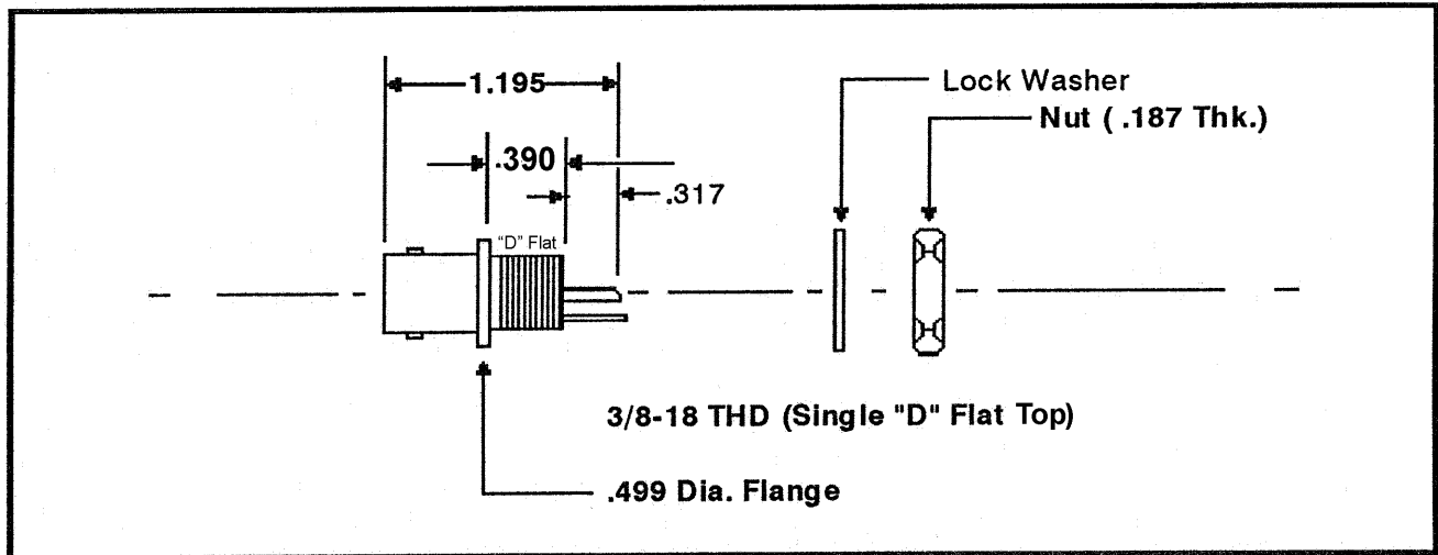
BNC Jack, Panel Mount (Isolated) P/N 326R515 Series
